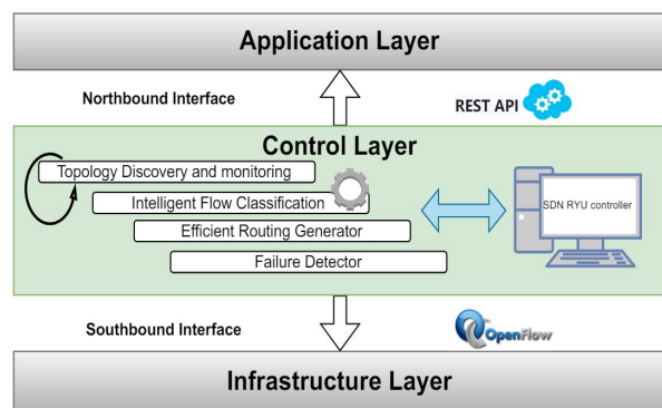
Fig. 2: HIFFR System Architecture with Post-Failure Management.
